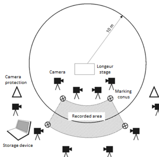
Picture 1. Sketch diagram of cameras layout and of other material equipment
